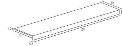
GRADINO PLUS BORDO** 34x120x4,5 cm Rect - 13 3/8 "x48"x1 3/4 " NATURALE ± 9 mm
